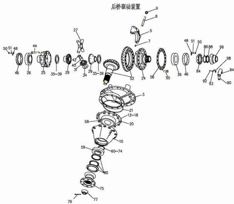
4.03 后桥驱动装置 (i=5.73, Φ165)/Drive of Rear Axle
